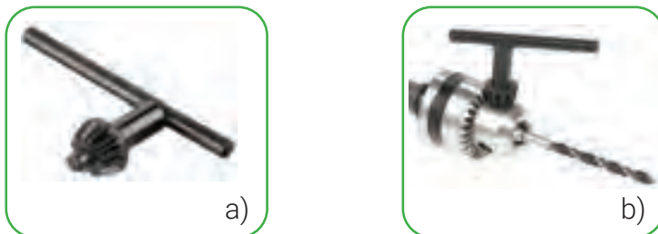
17-rasm. Parmani patronga o'rnatish jarayoni: a) kalit; b) patronga parmani o'rnatish.
