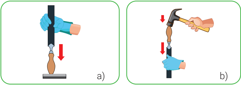
46-rasm. Egov dastasini o’rnatish: a) egovni dastaga o’rnatish; b) dastani egovga mustahkamlash;
